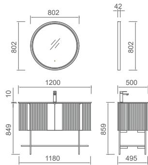
OJS246-1200 Main Cabinet: 1200x500x849mm Mirror: 802x42x802mm
