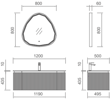
OJS243-1200 Main Cabinet: 1200x500x435mm Mirror: 800x60x800mm
