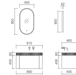
OJS264-900 Main Cabinet: 910x465x450mm Mirror: 450x42x850mm
